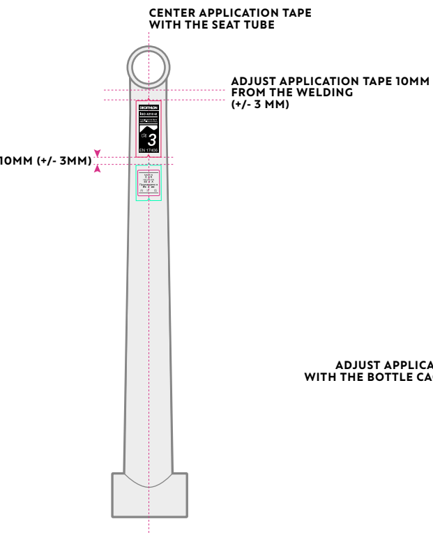
DOWNTUBE BOTTOM VIEW
