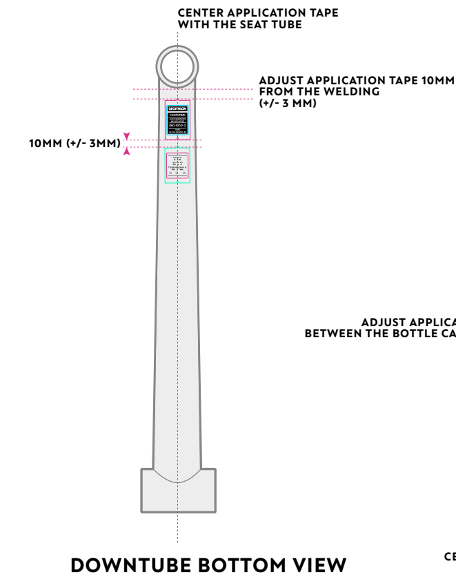
DOWNTUBE BOTTOM VIEW
