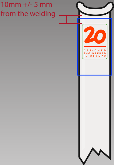
SEAT TUBE - FRONT VIEW
