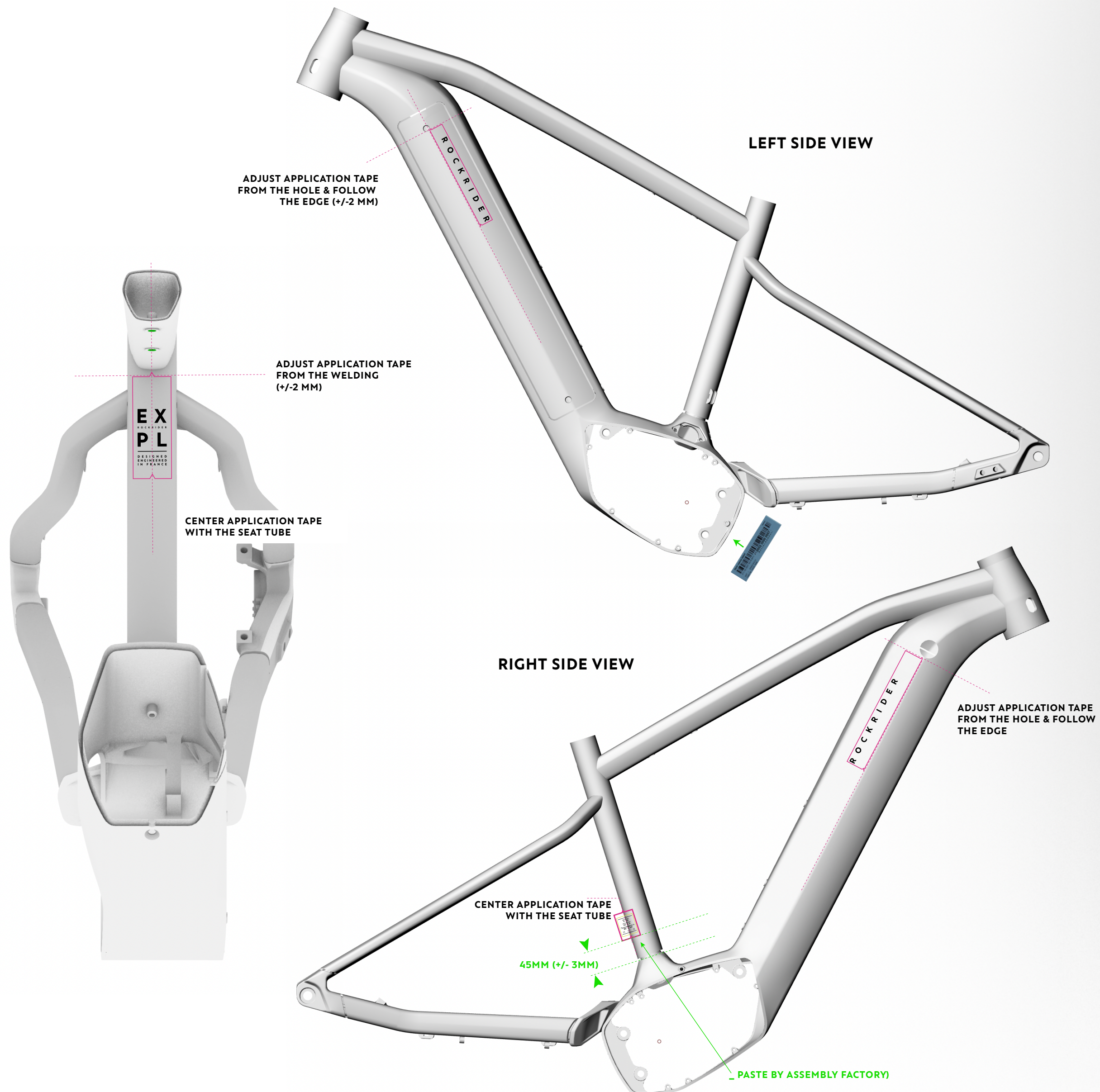
DOWNTUBE TUBE TOP VIEW
