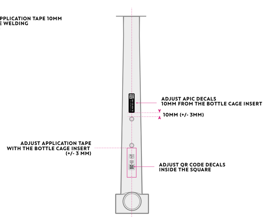
DOWNTUBE TOP VIEW
