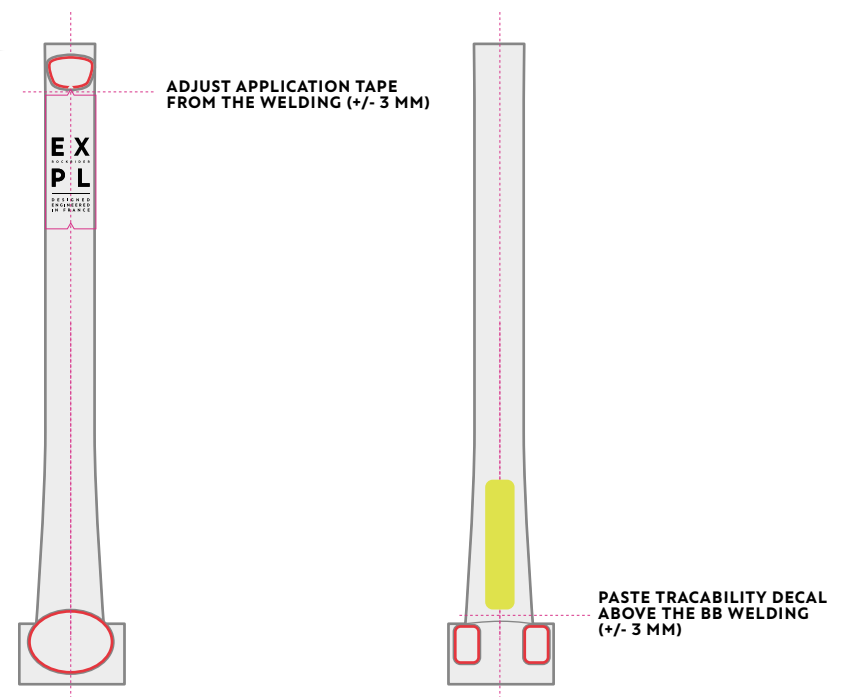
SEATTUBE FRONT VIEW
