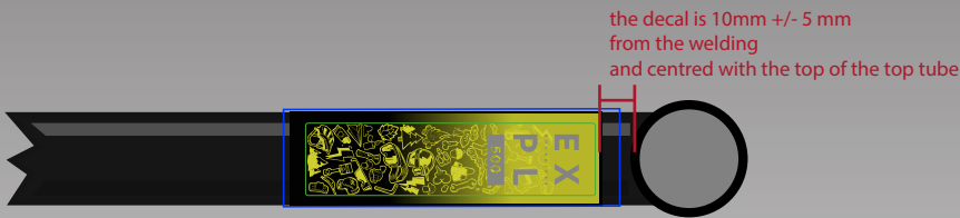
TOP TUBE - TOP VIEW
