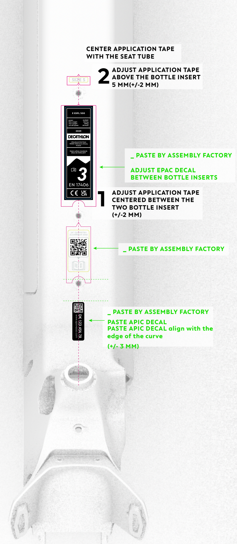
DOWNTUBE TUBE TOP VIEW
