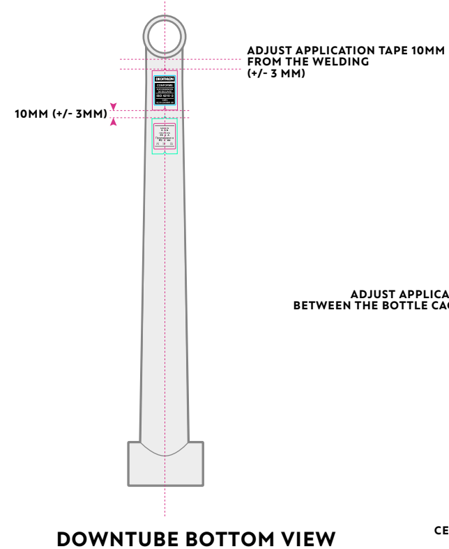
DOWNTUBE BOTTOM VIEW
