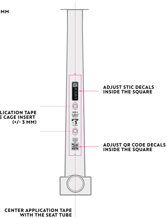
DOWNTUBE TOP VIEW
