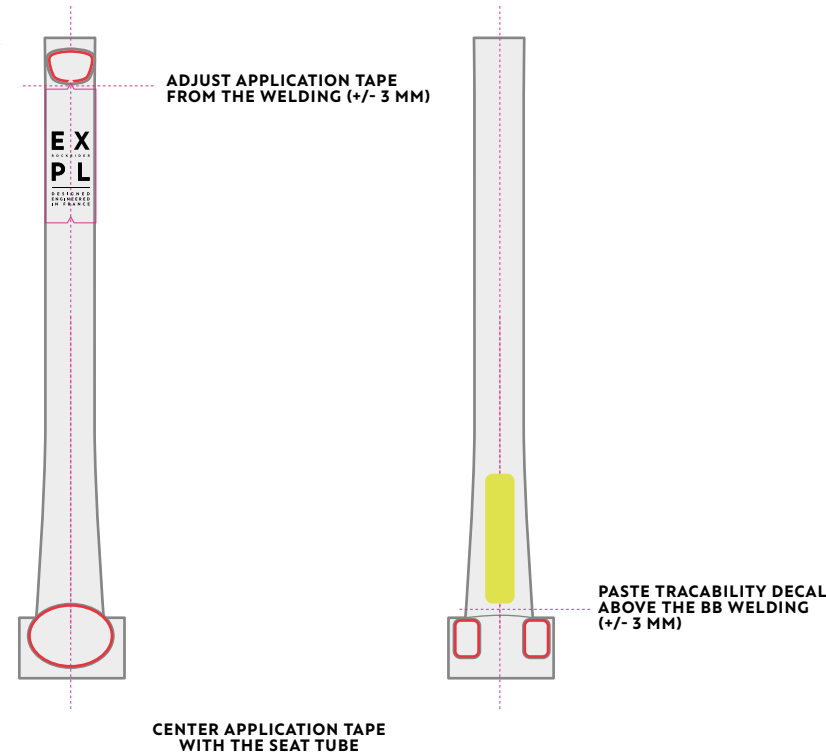
SEATTUBE FRONT VIEW
